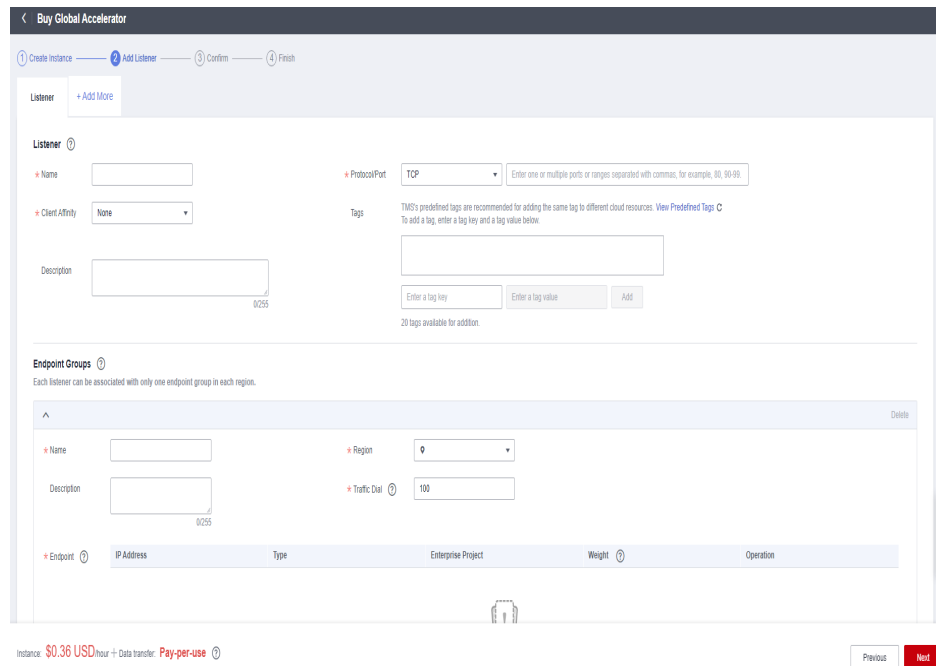
Figure 1-2 Adding a listener
